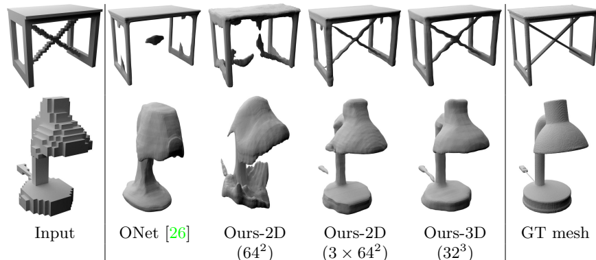
Fig. 4: Voxel Super-Resolution. Qualitative comparison between our method and ONet using coarse voxelized inputs at resolution 32^3 voxels.
