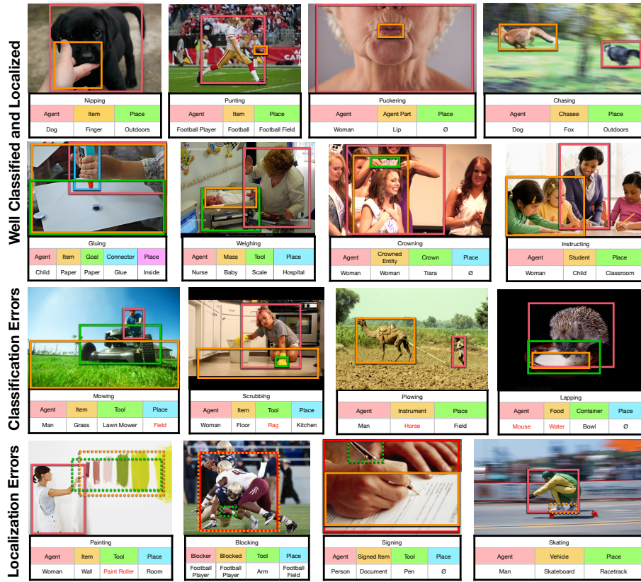
Fig. 9. Qualitative results for the proposed JSL model. First two rows show examples with correctly classified situations and detected groundings; and demonstrates the diversity of situations in the data. Third row shows classification errors. Note that some of them are perfectly plausible answers. Fourth row shows incorrect groundings; some of which are only partially wrong but get counted as errors nonetheless
