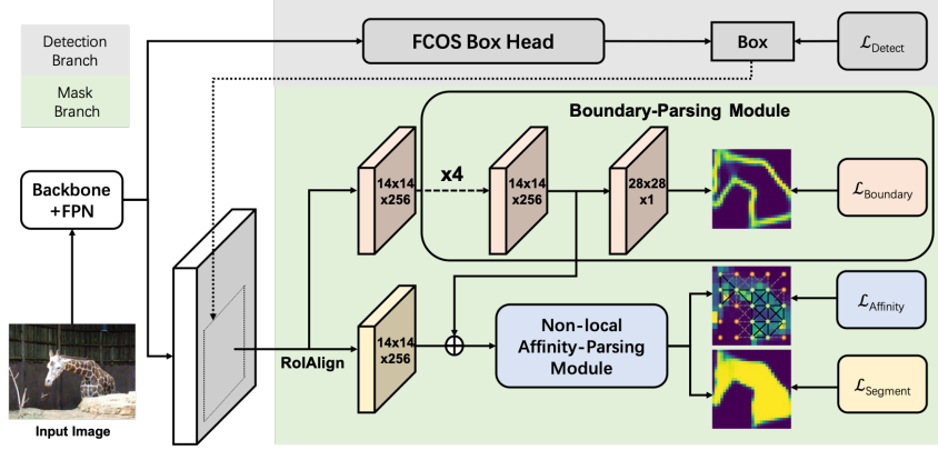
Fig. 2. Architecture of our Commonality-Parsing Network.
