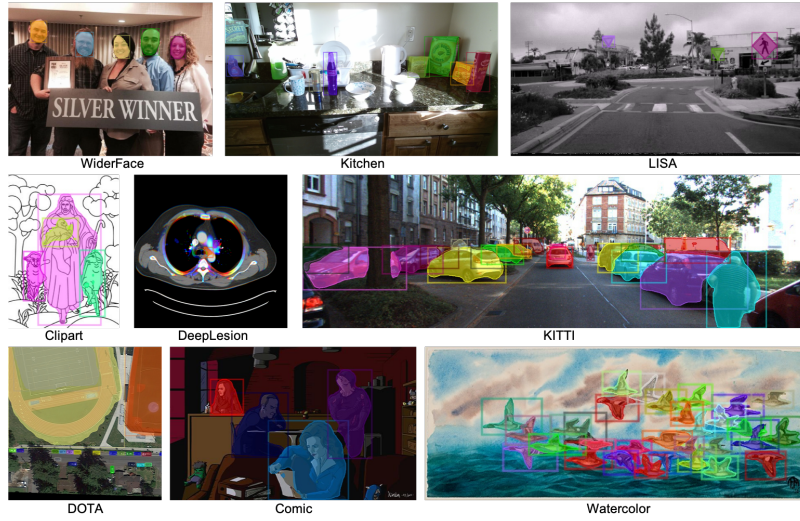
Fig. 7. Qualitative results of generalization by our model to 9 different datasets. The model is only trained on COCO and directly applied on these datasets.
