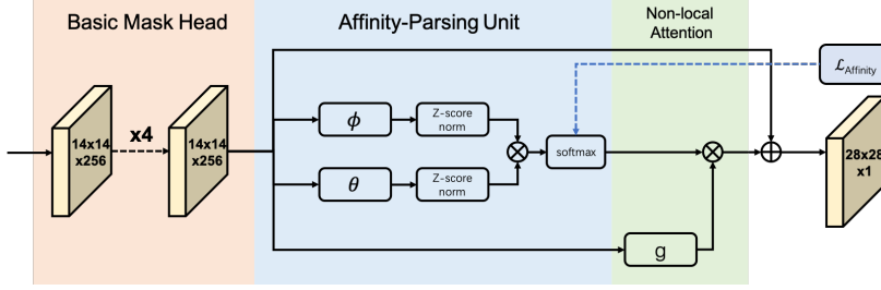
Fig. 3. Architecture of our Non-local Affinity-Parsing Module.
