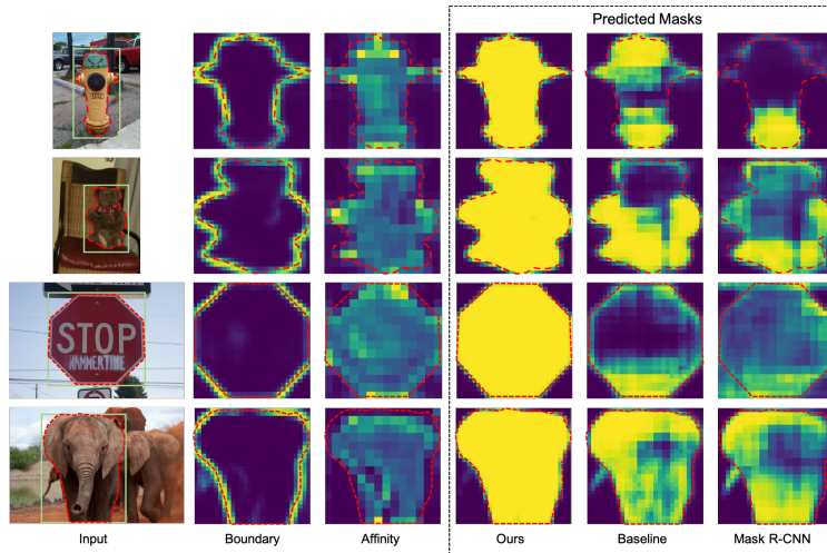
Fig. 4. Visualization of boundary heatmaps and affinity heatmaps learned by our model for four novel categories of cases. The red dash lines indicate the ground-truth mask.
