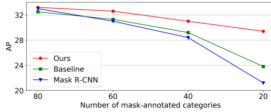
Fig. 5. The segmentation performance of different models on a fixed set of novel categories as a function of number of mask-annotated (base) categories. The novel categories are randomly selected from COCO dataset.
