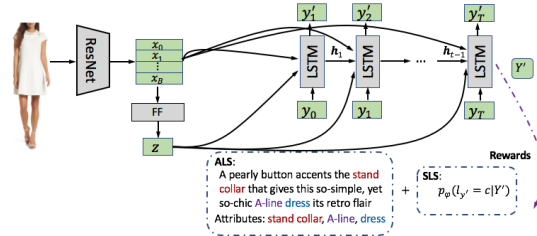
Fig. 3: The proposed model architecture and rewards.
