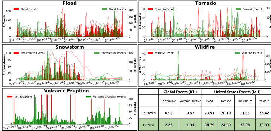
Fig.8. Temporal tweet filtering results. (Rows 1-2) For frequent events in the United States, we filter tweets for floods, tornadoes, snowstorms, and wildfires images and compare with ground truth frequency events obtained from NOAA. (Bottom Left) Filtered volcanic eruption images with ground truth events. (Bottom Right) Reported mRTI for global events and IoU for common US events.
