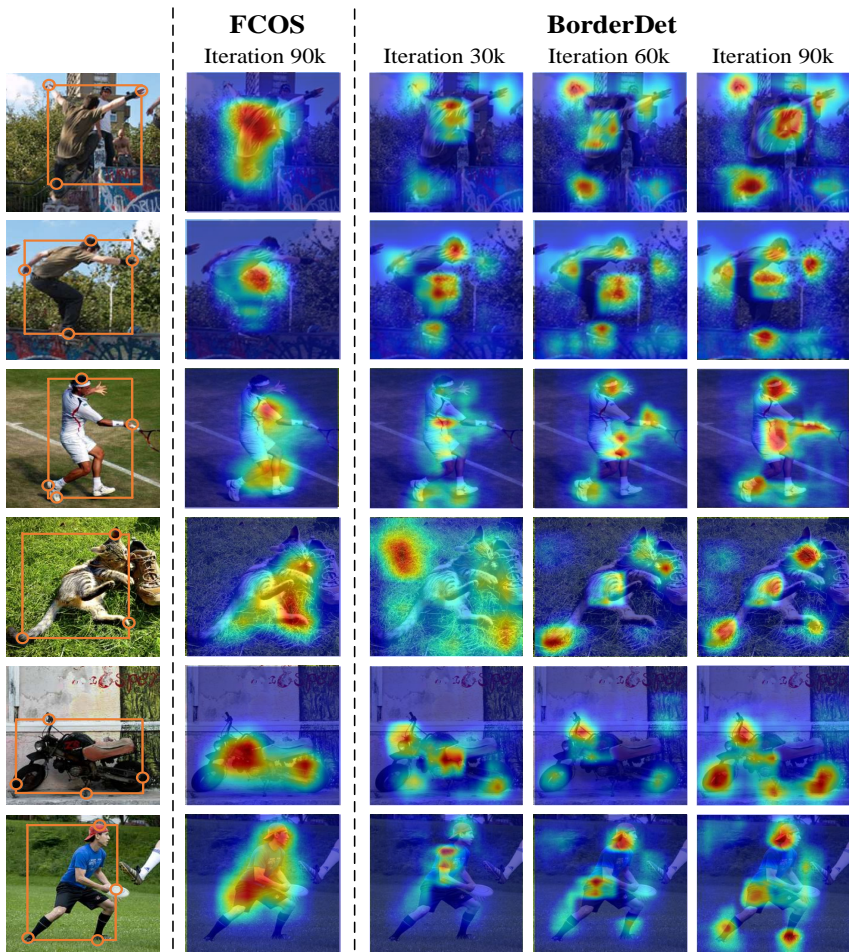
Fig. 1. visualization results of the border-sensitive feature maps. BorderDet is able to adaptively learn to extract the feature near location of the extreme point . These results further demonstrate the effectiveness of the proposed BorderDet for border feature extraction
