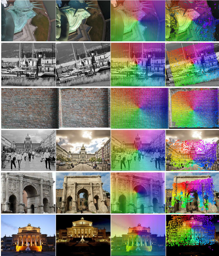
Fig. 2: Dense Correspondence. For each row, the first two columns show original images, and the last two columns show the correspondences found by our method. Colors indicate correspondences. The first and second three pairs of images are from HPatches [1] and MegaDepth [8], respectively. For each query point in the first image, we find its correspondence in the second image by nearest neighbor search using our dense descriptors. For the ease of visualization, we show correspondences for query points with an interval of 50 pixels on regular image grids.
