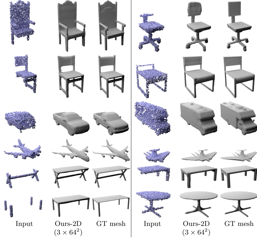
Fig. 4. Object-Level 3D Reconstruction from Partial Point Clouds. We show qualitative results on the ShapeNet “plane”, “car”, “chair” and “table” categories. Our method is able to correctly reconstruct 3D shapes from partial point clouds. Note that the models are trained on all classes.
