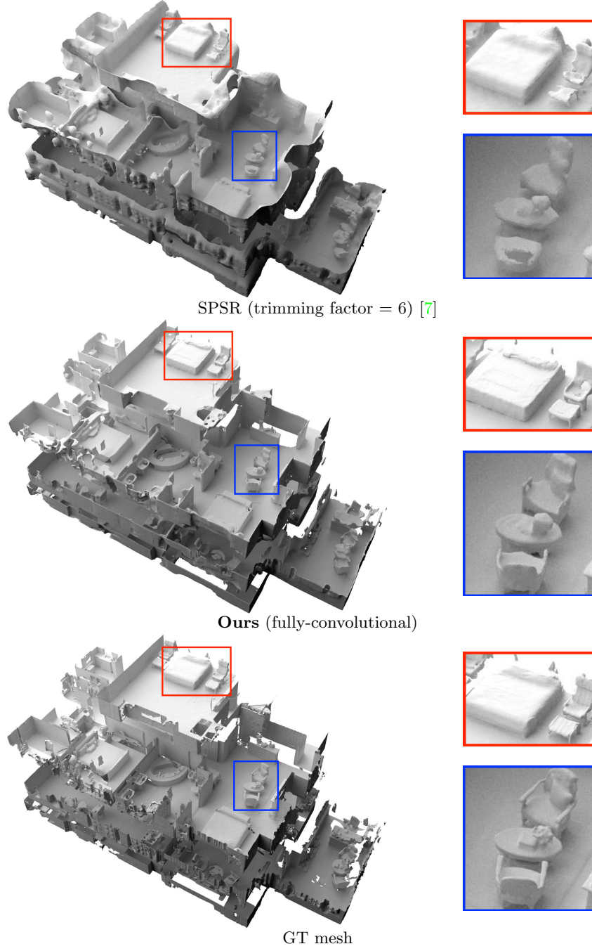
Fig. 7. Comparison of Building-Level Reconstruction on Matterport3D. Scene size: 19.7\text{m} \times 10.9\text{m} \times 9.4\text{m} . 200K points are sampled from the GT mesh and used as the input to SPSR and our method.
