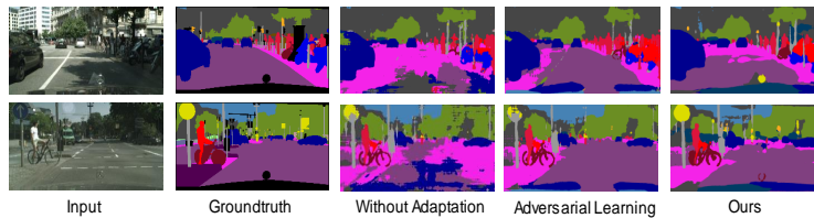
Fig. 2. Some qualitative results on SYNTHIA → Cityscapes task.
