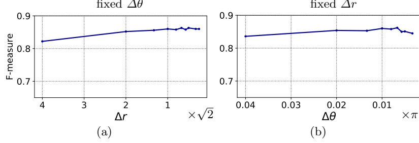
Fig. 7. (a): Performance under different distance quantization intervals \Delta r with a fixed angular quantization interval \Delta\theta = \pi/100 . Larger \Delta r indicates smaller quantization levels R . (b): Performance under different angular quantization intervals \Delta\theta with a fixed distance quantization interval \Delta r = \sqrt{2} .
