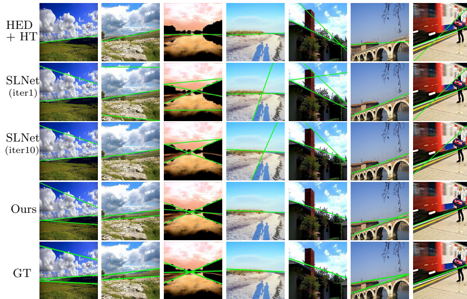
Fig. 9. Example detection results by different methods. Compared to SLNet [29] and classical Hough transform [11], our results are more consistent with the ground-truth.
