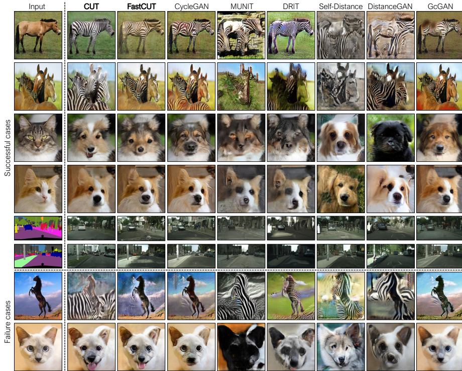
Fig. 3: Results. We compare our methods (CUT and FastCUT) with existing methods on the horse→zebra, cat→dog, and Cityscapes datasets. CycleGAN [81], MUNIT [40], and DRIT [37], are two-sided methods, while SelfDistance, DistanceGAN [3], and GcGAN [16] are one-sided. We show successful cases above the dotted lines. Our full version CUT is able to add the zebra texture to the horse bodies. Our fast variant FastCUT can also generate competitive results at the least computational cost of training. The final rows show failure cases. In the first, we are unable to identify the unfamiliar pose of the horse and instead add texture to the background. In the second, the method hallucinates a tongue.
