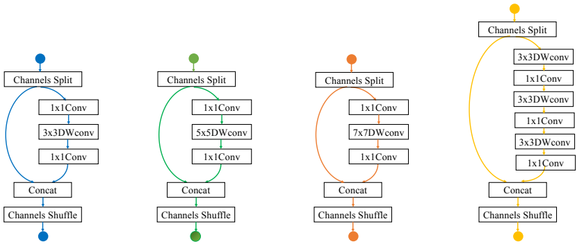
(a) Choice blocks with stride=1
