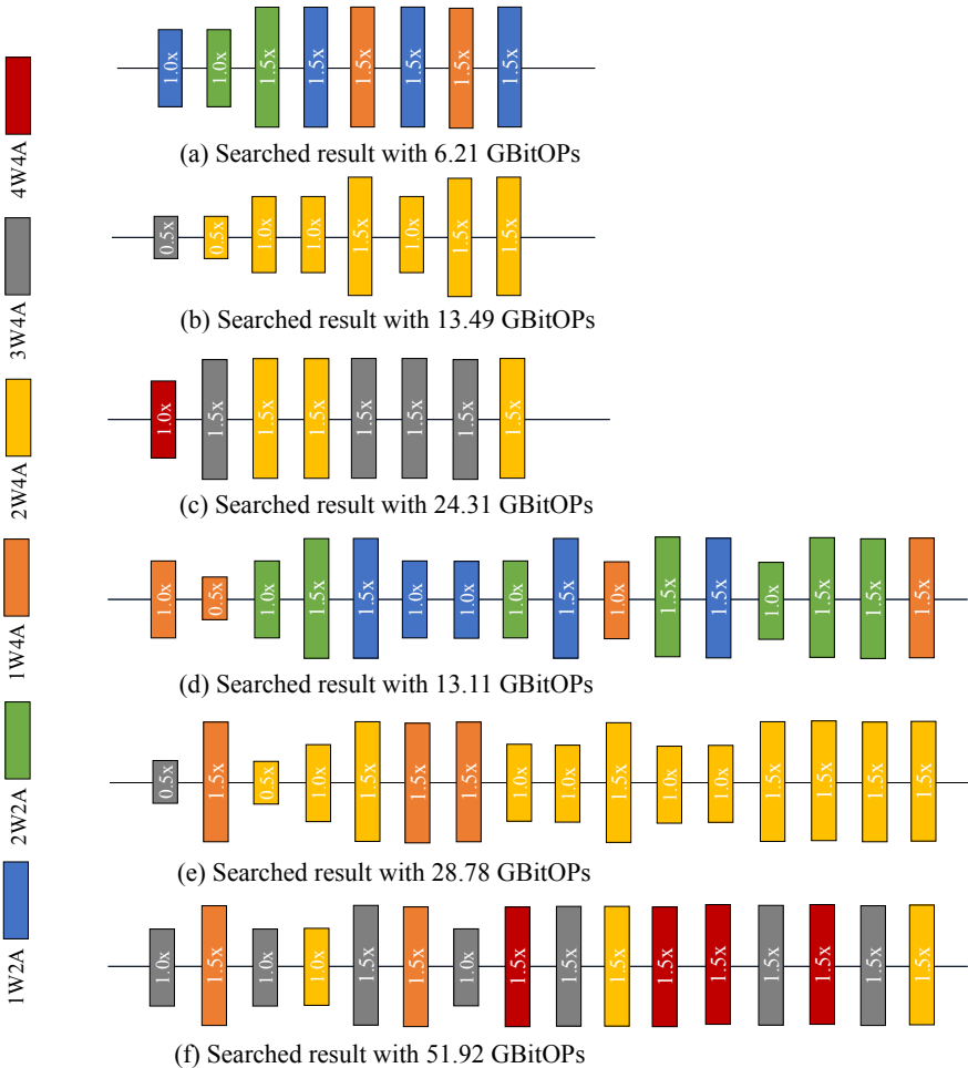
Fig. 5. Searched architectures of joint searching channel size and bit width under BitOPs constraints. (a) - (c) are searched based on Resnet18. (d) - (f) are searched based on Resnet34.
