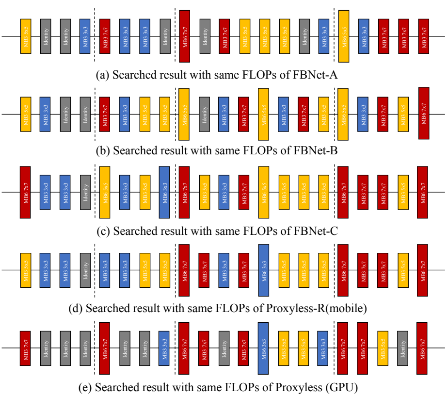
Fig. 3. Structures of searched architectures under FLOPs constraints by using ProxylessNAS search space.
