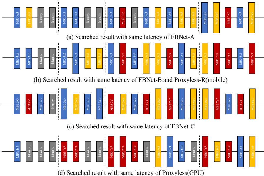
Fig. 4. Structures of searched architectures under GPU latency constraints by using ProxylessNAS search space.
