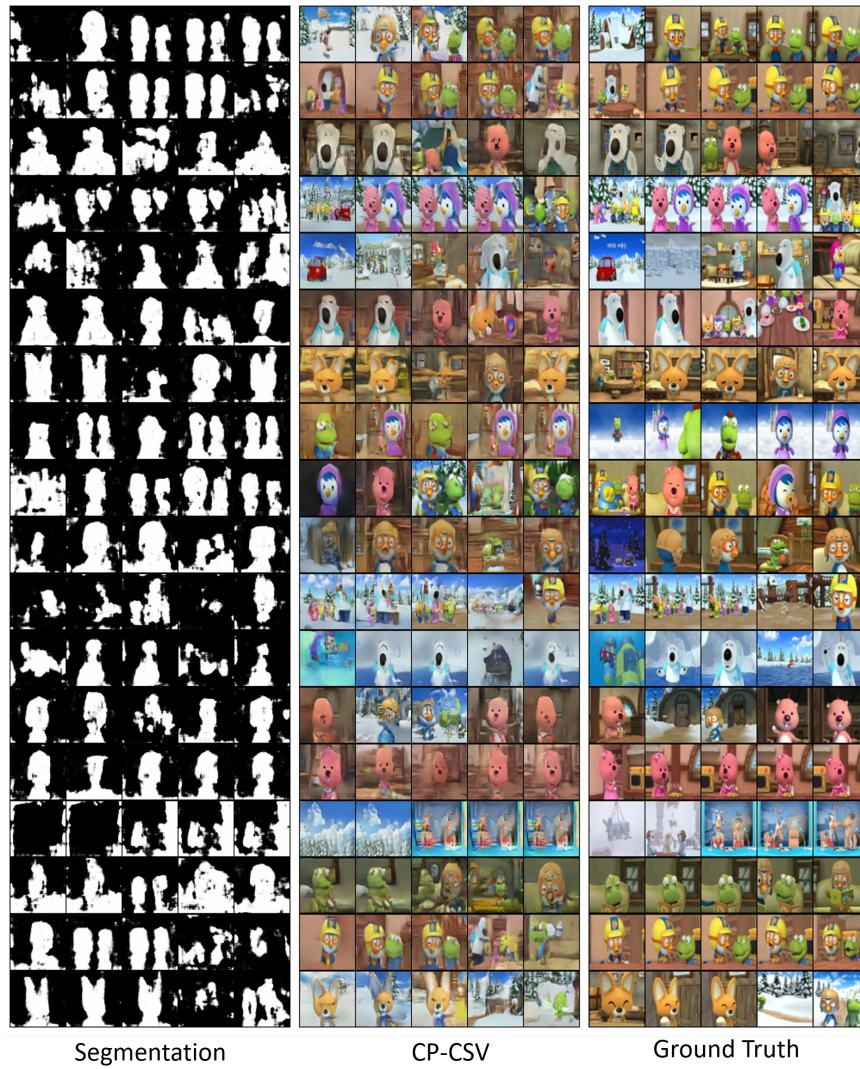
Fig. 7: Left two columns are the generated segmentation and image sequences of CP-CSV on Pororo-SV test dataset, and the ground truths are on the right side.
