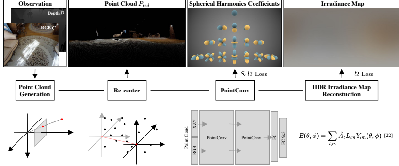
Fig. 3. PointAR pipeline composition and components. We first transform the camera view into a point cloud centered at the observation position, as described in Section 4.1. Then we use a compact neural network described in Section 4.2 to estimate SH coefficients at the rendering position. We use l_2 loss on both estimated SH coefficients and HDR irradiance map reconstructed from spherical harmonics coefficients for evaluation.
