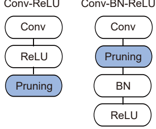
Fig. 1: Pruning stages involved for two typical structures: Conv-ReLU and Conv-BN-ReLU .
