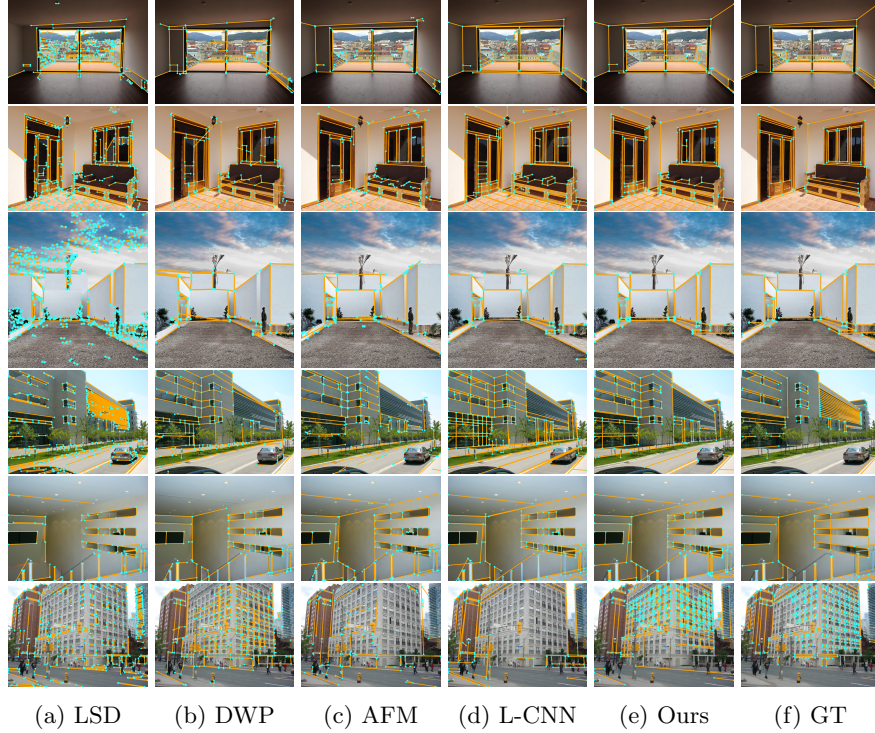
Fig. 8: Qualitative evaluation of line detection methods on Wireframe dataset and YorkUrban dataset. The line segments and their end-points are marked by orange and cyan colors, respectively.
