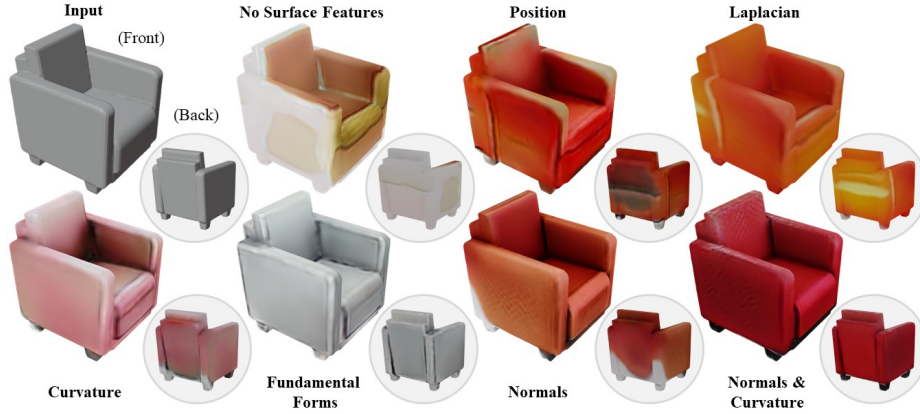
Fig. 7. Effect of different input surface features. Using no surface features (i.e. no surface encoder, only the decoder) produces poor textures since the decoder has limited understanding of the shape. 3D location based features such as position and Laplacian suffer from the inability to effectively align texture patterns with geometric ones. Curvature and fundamental forms introduce spurious line effects due to strong correlation with curvature. Surface normal are quite effective, and are further stabilised when used along with curvature.
