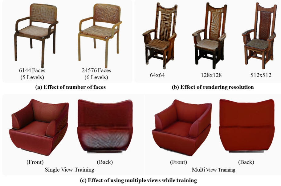
Fig. 8. (a) Increased mesh resolution enables synthesis of higher quality texture. (b) Higher rendering resolution during training helps synthesize more details. (c) Using a single viewpoint per mesh for discrimination can introduce artifacts in the texture across different regions of the mesh. In contrast, using multiple views instead encourages more coherent textures across views.
