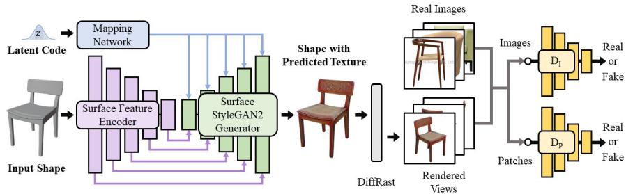
Fig. 2. Texturify Overview. Surface features from an input 3D mesh are encoded through a face convolution-based encoder and decoded through a StyleGAN2-inspired decoder to generate textures directly on the surface of the mesh. To ensure that generated textures are realistic, the textured mesh is differentially rendered from different view points and is critiqued by two discriminators. An image discriminator D_I operates on full image views from the real or rendered views, while a patch-consistency discriminator D_P encourages consistency between views by operating on patches coming from a single real view or patches from different views of rendered images.
