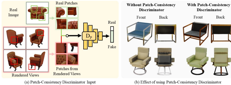
Fig. 4. The patch-consistency discriminator encourages global consistency in generated shape textures across multiple views. (a) While for real image data we are only considering patches from the same view (since the 2D image dataset does not contain multi-view data), we use patches from multiple views in the scenario of generated images. (b) Without patch-consistency discriminator rendered texture can end up having inconsistent styles across viewpoints. Using the patch consistency discriminator prevents this issue.
