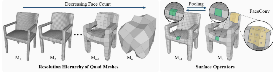
Fig. 3. Texturify generates textures on 4-RoSy parameterized quad meshes, where we define face convolutions with pooling and unpooling operations to operate on a hierarchy of the quad meshes. This enables reasoning about local surface neighborhoods across multiple resolutions to obtain effective global structures as well as fine details.
