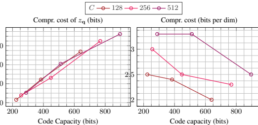
Fig. 7: Cost of compressing z_q using the GPT, in bits and bits per dimension.
