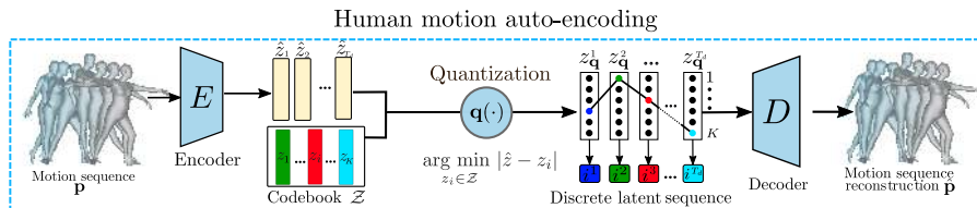
Fig. 2: Discrete latent representation for human motion. The encoder E maps a human motion \mathbf{p} to a latent representation \hat{z} which is then quantized using a codebook \mathcal{Z} . The decoder D reconstructs the human motion \hat{\mathbf{p}} from the quantized latent sequence \mathbf{z}_q .
