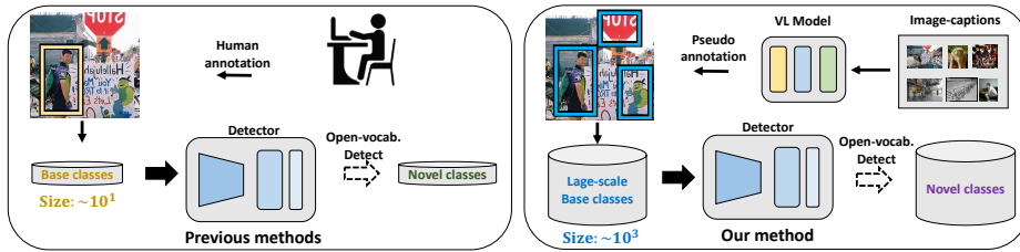
Fig. 1. Previous methods (left) rely on human-provided box-level annotations of pre-defined base classes during training and attempt to generalize to objects of novel classes during inference. Our method (right) generates pseudo bounding-box annotations from large-scale image-caption pairs by leveraging the localization ability of pre-trained vision-language (VL) models. Then, we utilize them to improve our open vocabulary object detector. Compared to the human annotations of a fixed/small set of base classes, our pseudo bounding-box label generator easily scales to a large set of diverse objects from the large-scale image-caption dataset, thus is able to achieve better detection performance on novel objects compared to previous methods
