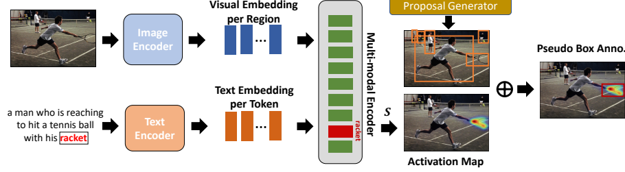
Fig. 2. Illustration of our pseudo box label generation process. The input to the system is an image-caption pair. We use image and text encoders to extract the visual and text embeddings of the image and its corresponding caption. We then obtain multi-modal features by image-text interaction via cross-attention. We maintain objects of interest in our pre-defined object vocabulary. For each object of interest embedded in the caption (for example, racket in this figure), we use Grad-CAM to visualize its activation map in the image. This map indicates the contribution of the image regions to the final representation of the object word. Finally, we determine the pseudo bounding-box label of the object by selecting the object proposal that has the largest overlap with the activation
