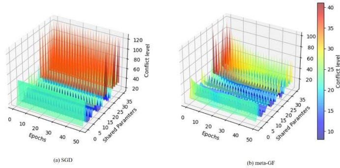
Fig.1 Gradient conflict
