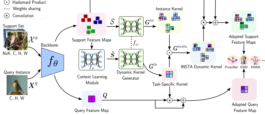
Fig. 2: The framework of our method. Given the support set \mathcal{X}^s and the query sample X^q , the backbone network f_\theta first encodes them into a representation space as \mathcal{S} = \{\mathcal{S}_{11}, \dots, \mathcal{S}_{NK}\} and Q . Then a dynamic generator f_\omega is used to produce an instance kernel for each support sample. Meanwhile, a context learning module f_\phi is used to refine and aggregate the context of the entire support feature maps to produce a task-specific representation, which is then used as the input of f_\omega to obtain the task-specific kernel. Note the instance kernel and task-specific kernel share the parameters across f_\omega . Finally, the INSTA dynamic kernel that is both instance-aware and task-aware is applied to the support feature maps, while only the task-specific kernel is applied to the query feature map to obtain the adapted representations
