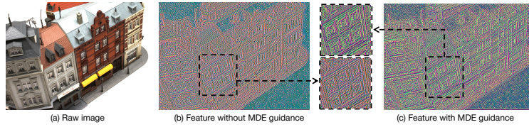
Fig. 4. An example shows that MDE guides the FPN feature to deliver more details at object boundaries. For better visualization, we leverage PCA to reduce the number of feature channels to 3 and color the channels with RGB.
