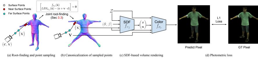
Fig. 2: Overview of Our Pipeline. (a) Given a ray (\mathbf{c}, \mathbf{v}) with camera center \mathbf{c} and ray direction \mathbf{v} in observation space, we jointly search for its intersection with the SDF iso-surface and the correspondence of the intersection point via a novel joint root-finding algorithm (Section 3.3). We then sample near/far surface points \{\bar{\mathbf{x}}\} . (b) The sampled points are mapped into canonical space as \{\hat{\mathbf{x}}\} via root-finding. (c) In canonical space, we run an SDF-based volume rendering with canonicalized points \{\hat{\mathbf{x}}\} , local body poses and shape (\theta, \beta) , an SDF network feature \mathbf{z} , surface normals \mathbf{n} , and a per-frame latent code \mathbf{Z} to predict the corresponding pixel value of the input ray (Section 3.4). (d) All network modules, including the forward LBS network LBS_{\sigma_w} , the canonical SDF network f_{\sigma_f} , and the canonical color network f_{\sigma_c} , are trained end-to-end with a photometric loss in image space and regularization losses in canonical space (Section 3.5).
