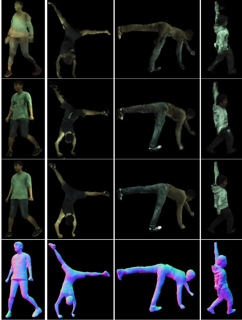
Fig. 5: Qualitative Results on Out-of-distribution Poses from the AMASS [40] and AIST++ [32] datasets. From top to bottom row: Neural Body, Ani-NeRF, our rendering, and our geometry. Note that Ani-NeRF requires re-training their backward LBS network on novel pose sequence. We did not show A-NeRF results as it already produces severe overfitting effects on ZJU-MoCap test poses. For more qualitative comparisons, please refer to the Supp. Mat.
