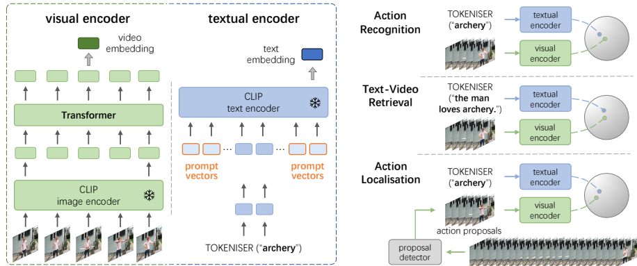
Fig. 1: Framework Overview. We prepend / append several learnable prompt vectors to the CLIP text encoder to generate action classifiers or embeddings; adopt a lightweight Transformer on top of the CLIP image encoder for temporal modeling. During training, both the image and text encoders are kept frozen . By optimising task-specific prompt vectors and temporal Transformer, we efficiently adapt CLIP to various video understanding tasks: action recognition, retrieval, and localisation, across closed-set, few-shot, and zero-shot scenarios.
