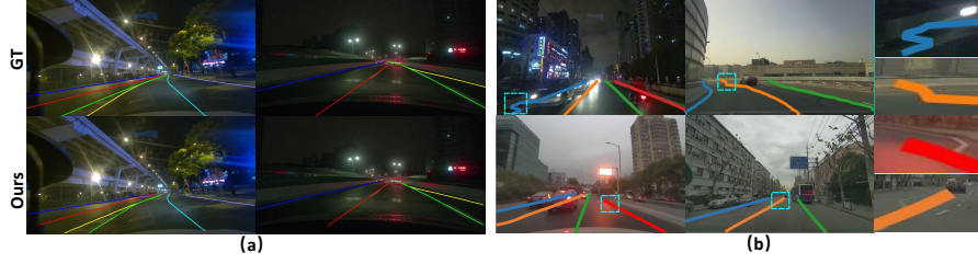
Fig. 1. Challenging scenes (curve lanes, Y-shape lanes). The first row of (a) shows the ground truth while the second row is our predictions. The first row of (b) shows the result of segmentation-based methods that global shape of lane is not well fitted. While the second row of (b) shows proposal-based methods, can not depict local locations of Y-shape and curve lanes.
