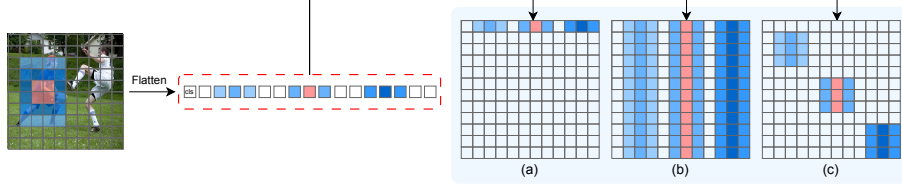
Fig. 8: Several ways to generate foveal attention masks. (a) Only assigning values at the position corresponding to the ROA token in the first row. (b) Assigning values of ROA token position in all rows. (c) Assigning values at the position corresponding to the ROA token on the diagonal line.
