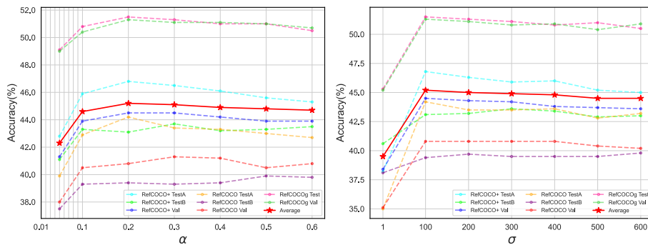
Fig. 9: Effect of \alpha and \sigma in masks. The accuracy peaks when \alpha = 0.2 , as it highlights the features of the specific object while preserving the contextual information. When \sigma = 1 , the concentration of values within a mask can lead to a lack of rich features in specific regions. We consider \alpha = 0.2 and \sigma = 100 as the optimal value.
