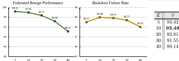
Fig. 3: Ablation on local epoch E on MNIST ( \gamma = 0.5 ) with \rho = 30\% for the federated benign performance A (Left), backdoor failure rate R (middle) and the trade-off V (Right). Refer to Sec. 4.2 for explanation.
