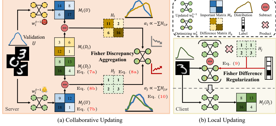
Fig. 1: Schematization of Self-Driven Fisher Calibration (Sec. 3.2). We utilize FIM to calculate parameter important matrix on local \mathcal{M}_k(D_k) and validation \mathcal{M}_k(U) distributions to measure importance difference H_k as \begin{bmatrix} 6 \\ 6 \end{bmatrix} = \begin{bmatrix} 6 \\ 6 \end{bmatrix} - \begin{bmatrix} 12 \\ 12 \end{bmatrix} / j . Fisher Difference Regularization (Sec. 3.2) regulates those parameters with large distinct importance. Fisher Discrepancy Aggregation (Sec. 3.2) allocates high aggregation weight for those with small parameter important discrepancy. We illustrate with network scale jWj=4 and class number jCj=5 . Best viewed in color. Zoom in for details.
