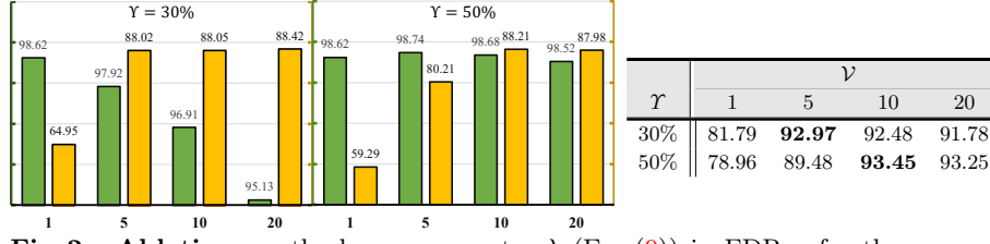
Fig. 2: Ablation on the hyper-parameter \lambda (Eq. (9)) in FDReg for the proposed method on MNIST with \gamma \in \{30\%, 50\%\} . \mathcal{A} (■) and \mathcal{R} (■). We default set \lambda=5 in the following experiments. Refer to Sec. 4.2 for detailed information.
