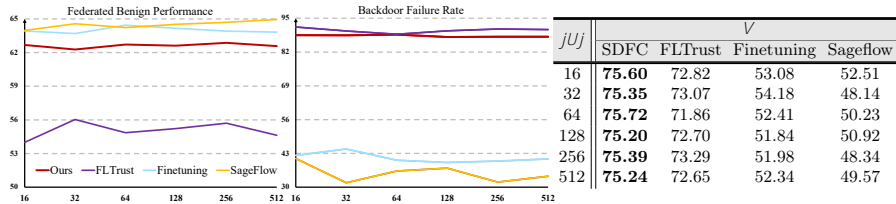
Fig. 4: Ablation on Validate Data Scale jUj in Cifar-10 ( \beta = 0.5 ; \gamma = 30\% ) with federated benign performance A (Left), backdoor failure rate R (middle) and the trade-off V (Right). Refer to Sec. 3.3.
