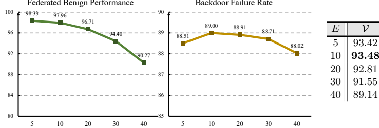
Fig. 3: Ablation on local epoch E on MNIST ( \beta = 0.5 ) with \Upsilon = 30\% for the federated benign performance \mathcal{A} (Left), backdoor failure rate \mathcal{R} (middle) and the trade-off \mathcal{V} (Right). Refer to Sec. 4.2 for explanation.
