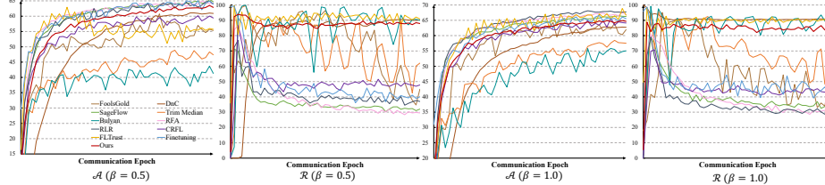
Fig. 7: Comparison of federated benign performance A and backdoor failure rate R during communication on Cifar-10 with \gamma = 30\% . SDFC appears stable convergence speed and satisfying performance. Please see details in Sec. 4.3.
