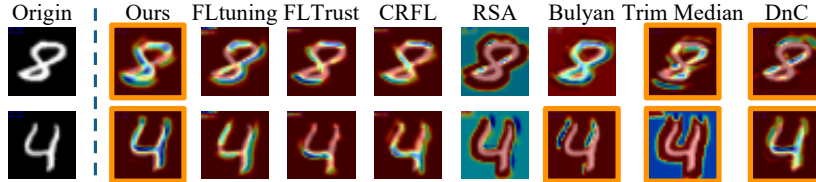
Fig. 6: Qualitative analysis under backdoor attack (Top Left) over MNIST ( \beta = 0.5 ; \gamma = 30\% ), where orange bound denotes corrected predictions. Refer to Sec. 4.3.
