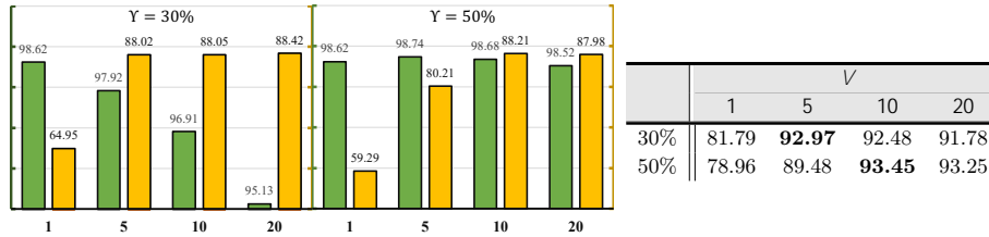
Fig. 2: Ablation on the hyper-parameter V (Eq. (9)) in FDRag for the proposed method on MNIST with \gamma \in \{30\%, 50\% . A ( \blacksquare ) and R ( \blacklozenge ). We default set \beta = 5 in the following experiments. Refer to Sec. 4.2 for detailed information.
