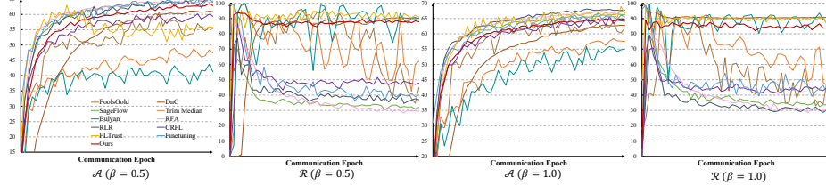
Fig. 7: Comparison of federated benign performance \mathcal{A} and backdoor failure rate \mathcal{R} during communication on Cifar-10 with \gamma = 30\% . SDFC appears stable convergence speed and satisfying performance. Please see details in Sec. 4.3.
