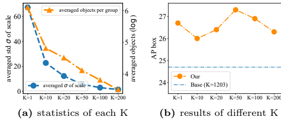
Fig. 3: The statistics (averaged standard deviation, averaged objects per group) of different K and its corresponding AP box.
