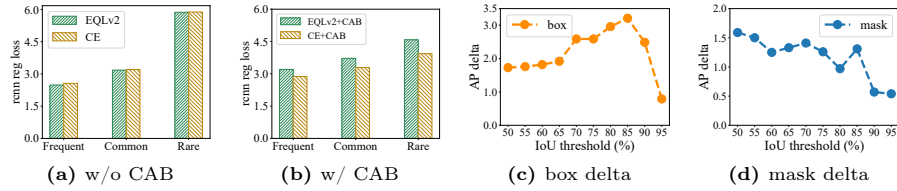
Fig. 5: The loss distribution shift before and after combining with our CAB (Fig. 5a, 5b), and AP improvement of combining our CAB with baseline in LVIS (Fig. 5c, 5d).
