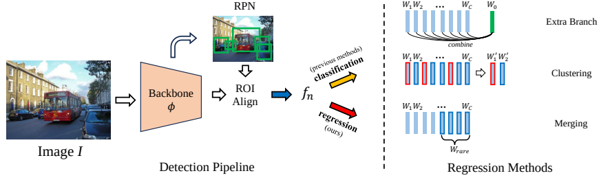
Fig. 2: Illustration of the regular two-stage detection pipeline and the proposed regression methods. Previous methods (the left figure) generally focus on the final classification branch (the yellow arrow), while we focus on rectifying the regression bias (the red arrow). The right part shows our three regression methods, including adding an extra branch W_0 , clustering regression heads ( e.g. , from W_1, \dots, W_C to W'_1, W'_2 ) and merging ( e.g. , merging rare categories into one regression head W_{rare} , cf. Table 2). In our main experiments, we choose ‘adding an extra branch’ for its simplicity. This figure needs to be viewed in color.
