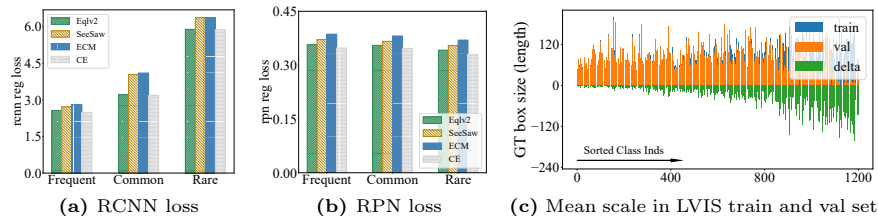
Fig. 1: 1a shows the RCNN regression train loss of frequent, common and rare categories. 1b shows the RPN regression loss. 1c shows distribution of per class mean object scales in LVIS1.0. ‘delta’ in 1c is the negative of difference between train and validation set sizes for different classes.
