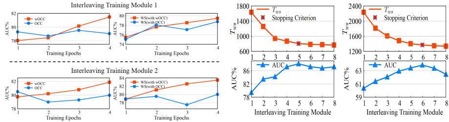
Fig. 3: Performance fluctuation in the first and second modules. Red line: AUC of mal. wOCC (or WS) when interleaving wOCC (or WS). Blue line: AUC of OCC (or WS) model in each module. Stars in top figures: when interleaving OCC and WS. Fig. 4: Left: ShanghaiTech. Right: UBnor. Top: T_{ws} in each interleaving training module. Bottom: The AUC of the WS model in each module. Stars in top figures: position where achieves stopping criterion.
